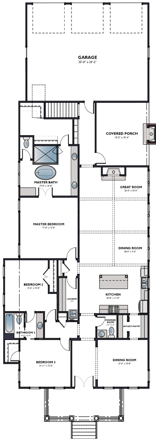
FIRST FLOOR
