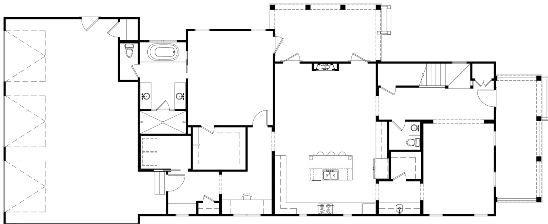
FIRST LEVEL FLOOR PLAN
